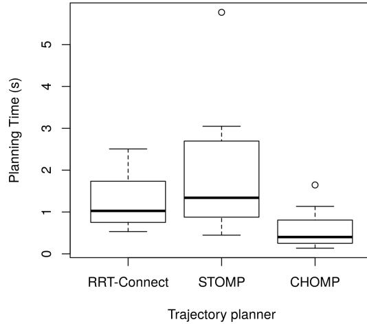
Figure 4.4: Planning Time for each trajectory planner on simulated scene I.
