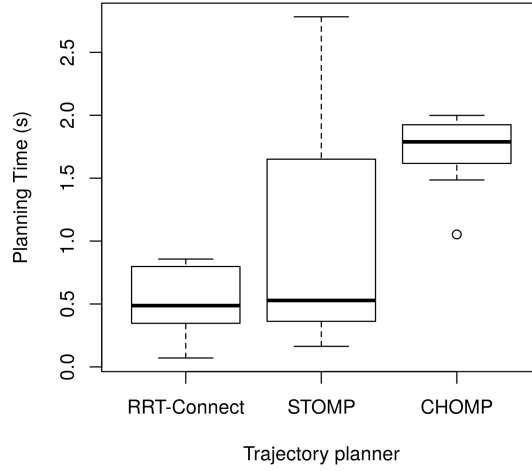
Figure 4.11: Planning Time for each trajectory planner on simulated scene III.
