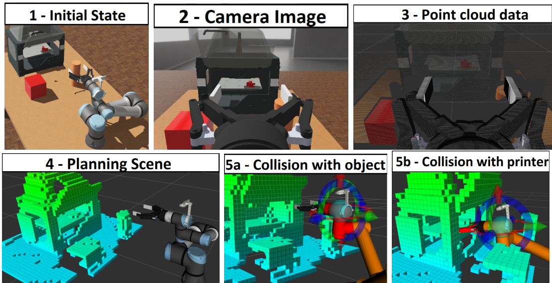
Figure 3.4: Obstacle collision detection pipeline.
